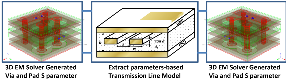
Figure 19: Cascade of the extracted transmission line model of the striplines and the S-parameters of the via and pad structures at both ends of the traces.
